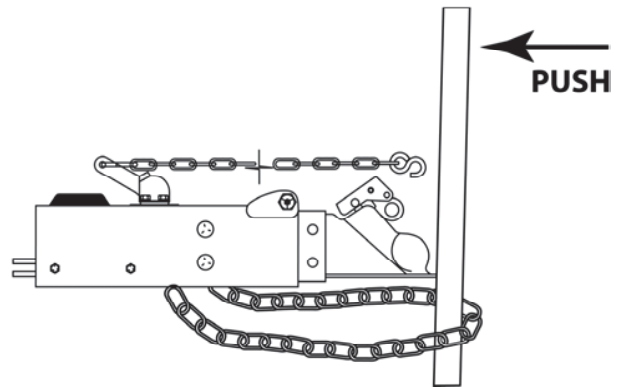
FIG. 2 - FIELD TEST SETUP
