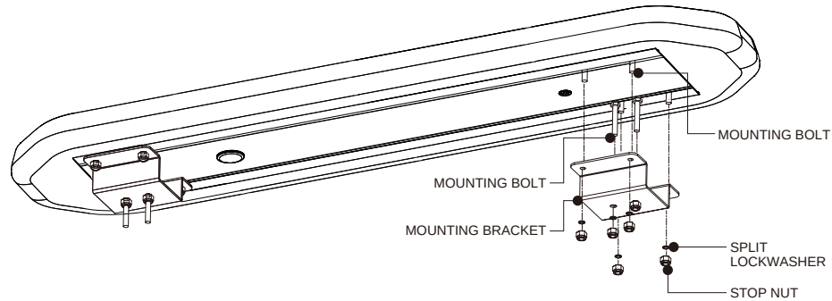
Hardware for Narrow Surface Mount
