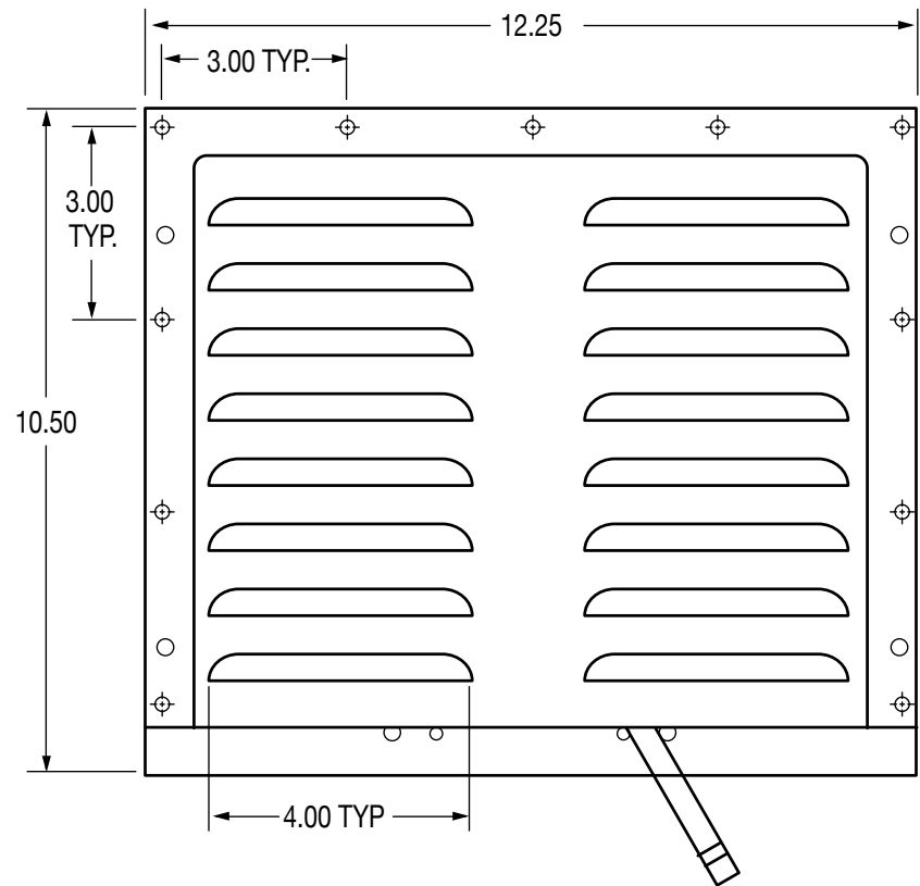
Adjustable Louvered Vent Shown
